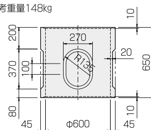
側塊6B
