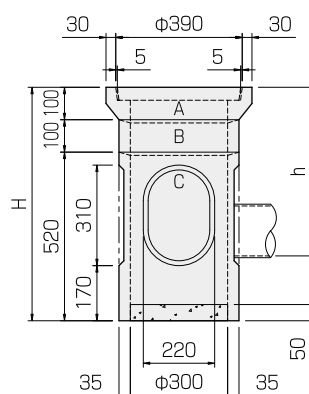
雨水桷(TMR30)
