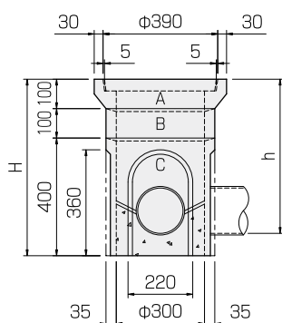
汚水桷(TMS30)
